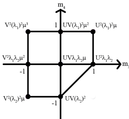
Figure 4. The dual polytope \Delta_{dP_2} and the associated monomials.
